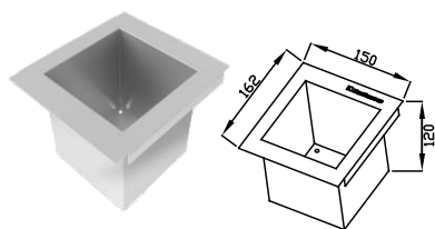
PORTA-DETERGENTE REF. 20.04.00125 • 150mm
